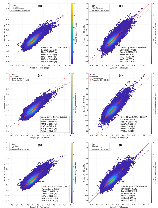
Figure 5. Scatter plots between tide gauges and baroclinic simulations for Grado with BC-ERA5 (a) and BC-UniGe (b), Monfalcone with BC-ERA5 (c) and BC-UniGe (d), and Trieste with BC-ERA5 (e) and BC-UniGe (f).
